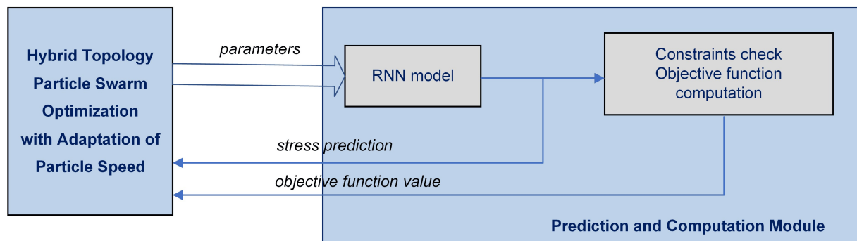
Figure 15: Structure of the Optimization Framework
